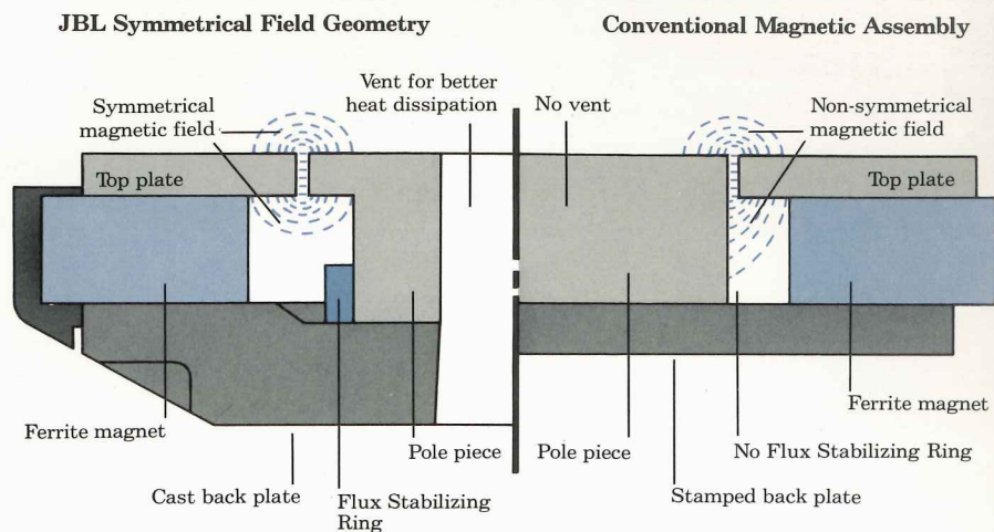
Cross-sections of JBL and conventional magnetic structures
