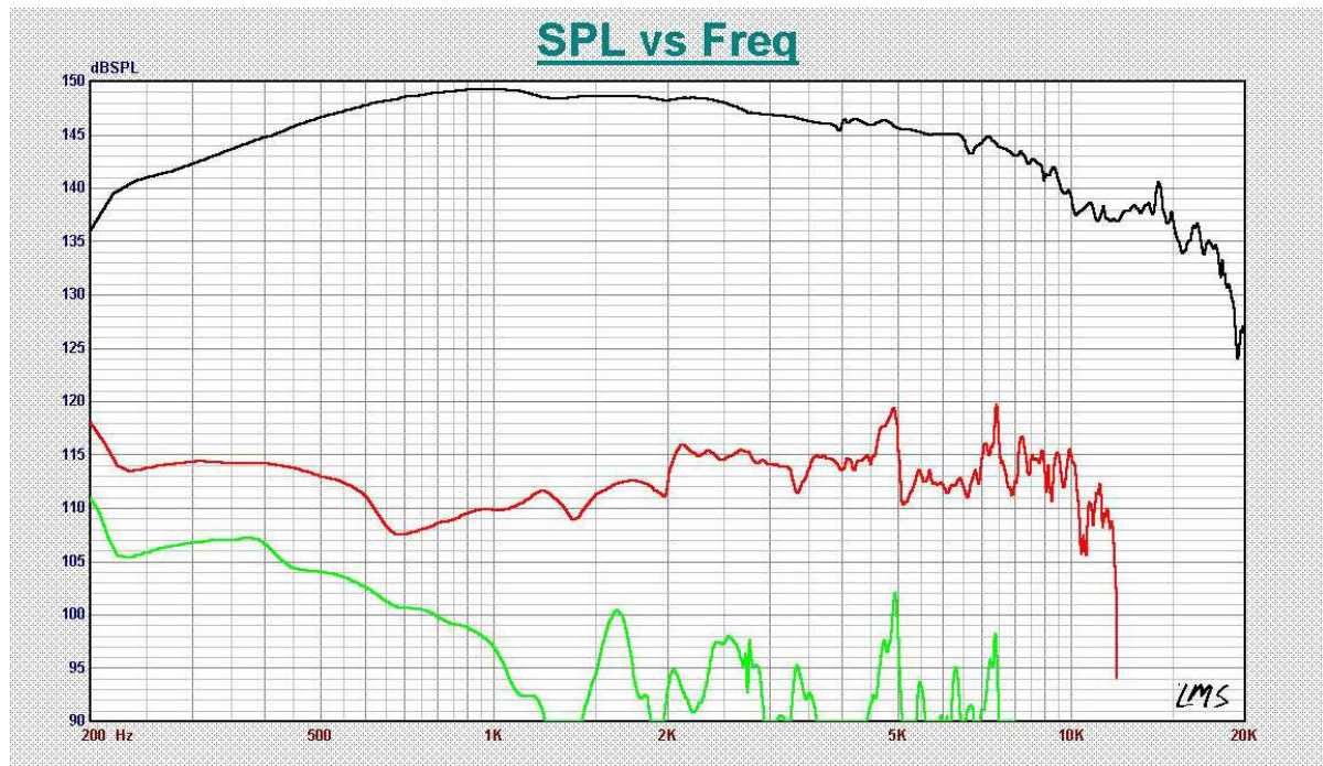
Figure 7 – Terminated tube measurement of 476Mg with distortion products. The measurement was made with 7.5 v applied to the driver. This is equates to about 120 dB @ 1m when mounted in the system.
