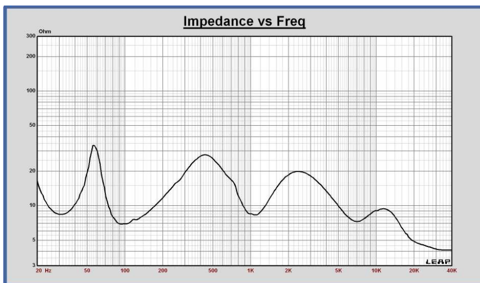
Figure 11 – Magnitude of impedance for the K2.S9900 system.
