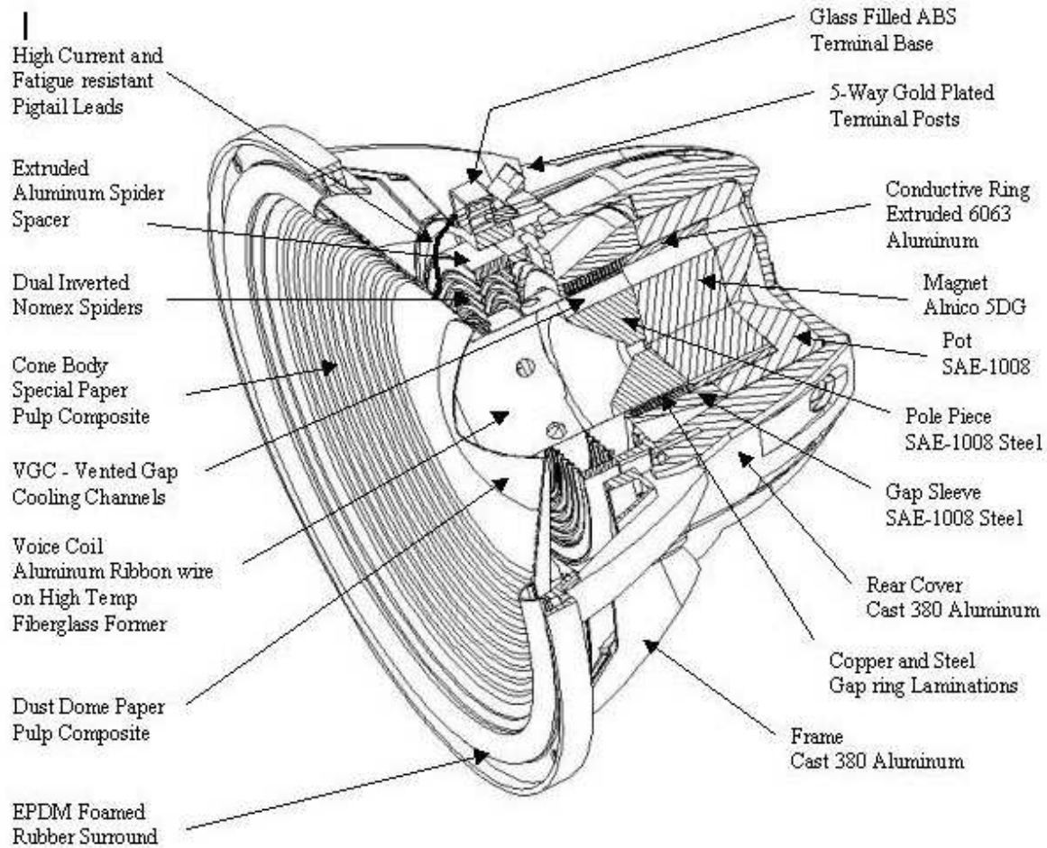
Figure 3 – 1500AL-1 section view
