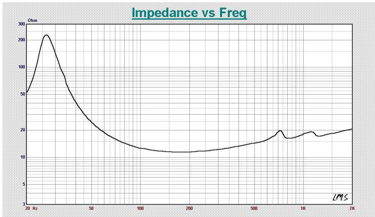
Figure 5 – 1500AL -1 Impedance curve in free air.
