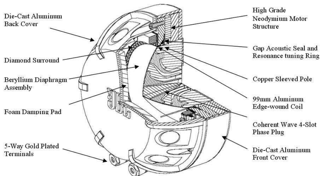
Figure 6 – 476Mg section view
