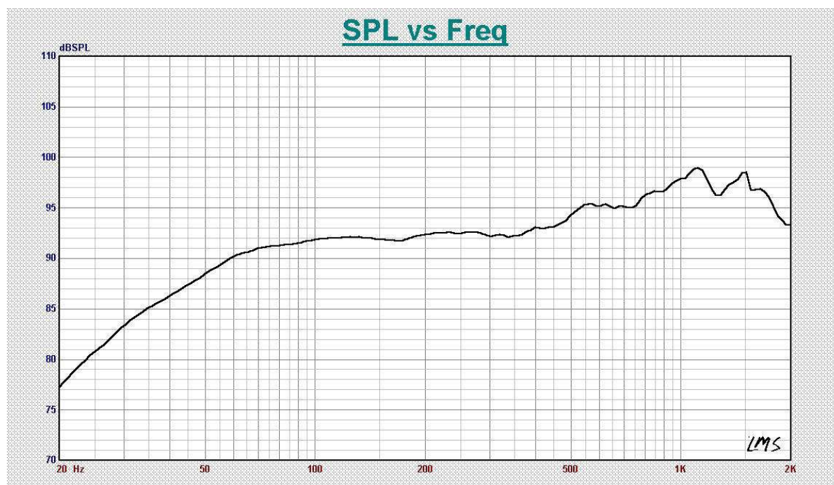
Figure 4 – 1500AL-1 half-space frequency response measured in a 19 cubic foot test enclosure. The measurement was made with 2.83 v @ 1m.
