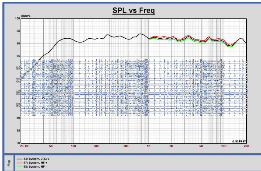
Figure 13 – Response changes due to HF Level adjustment 0.5 dB
